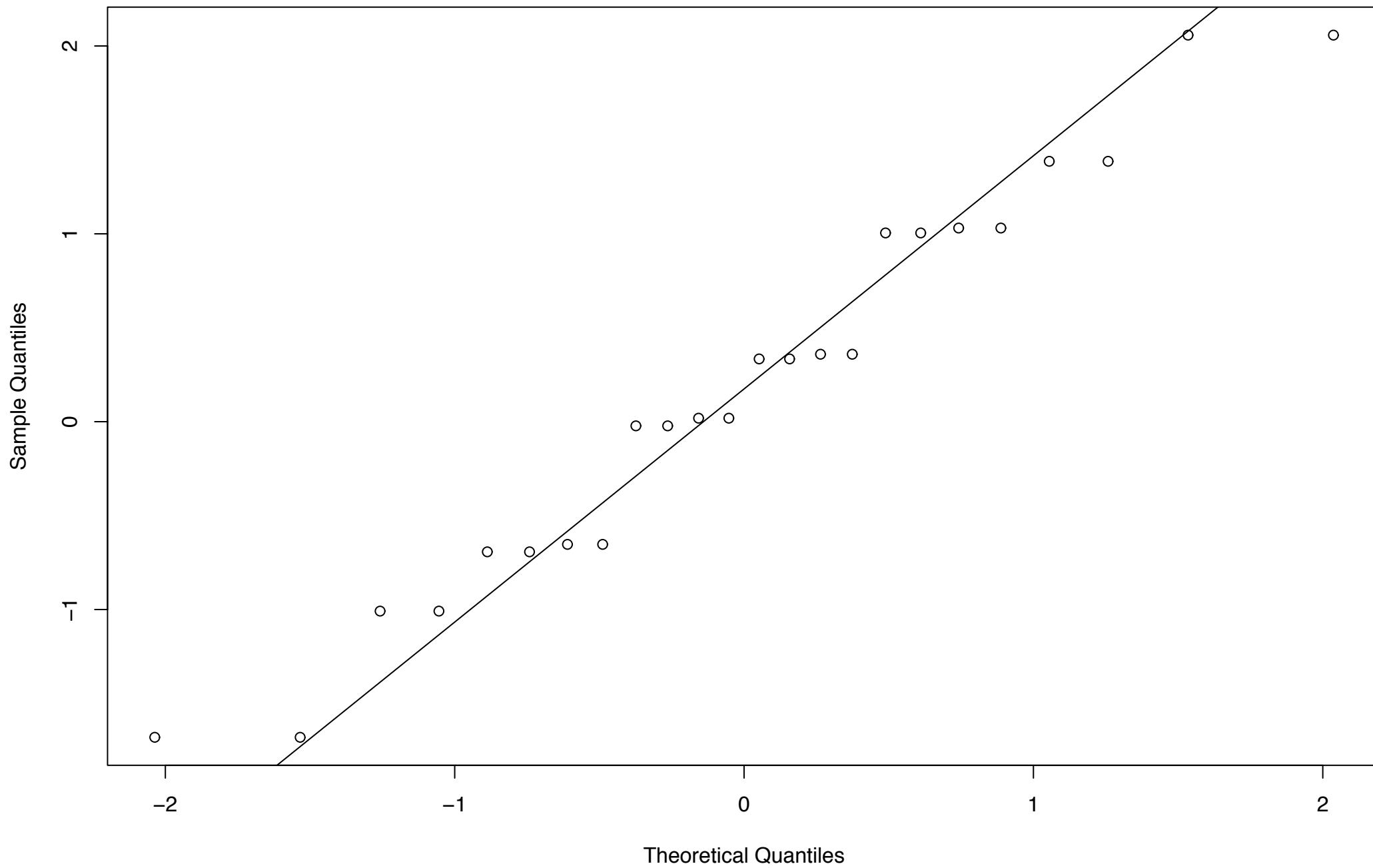
Normal Q-Q Plot
